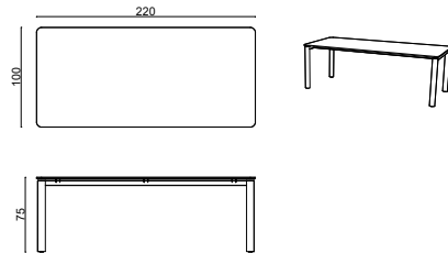
Layer Table - 100x220xh75 cm
