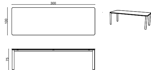
Layer Table - 100x300xh75 cm
