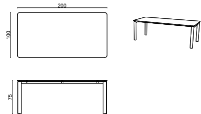
Layer Table - 100x200xh75 cm
