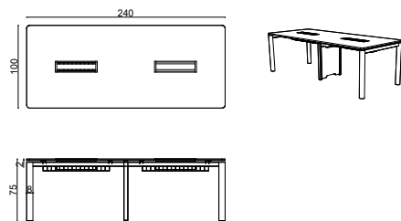
Layer Meeting Table - 100x240xh75 cm
