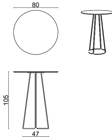
Nory Bar Table Ø80x H 105 cm
