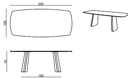
M. Allure Masa - 100x220xh75 cm
