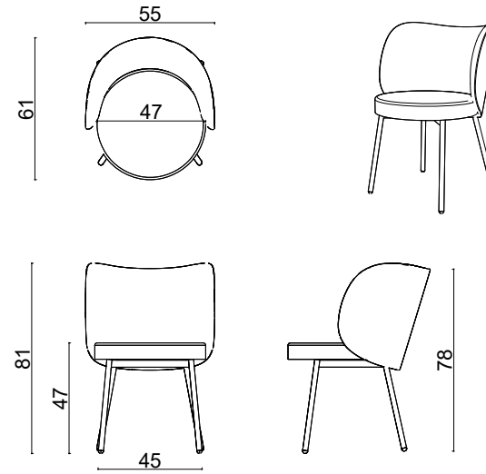
Birim Metal Chair
