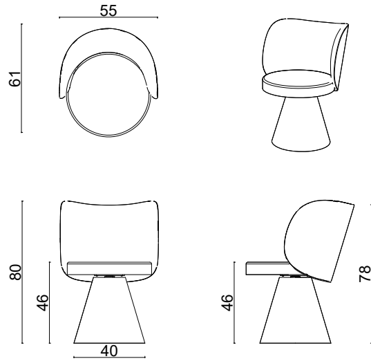
Birim Conical Chair
