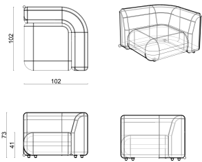
Corner 102x102 cm
