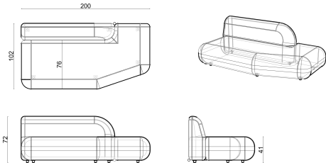
Open end Right 102x200 cm
