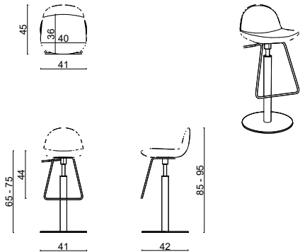
Rio Counter - Bar Height-Adjustable
