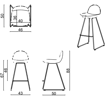
Rio Counter - Pipe Leg
