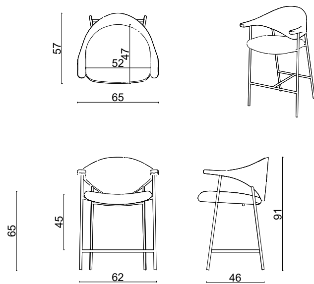
S.Trident Pipe Leg Counter
